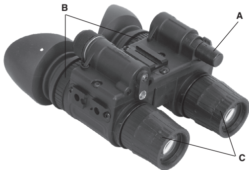
FIGURE 4-3. MECHANICAL FUNCTIONS
