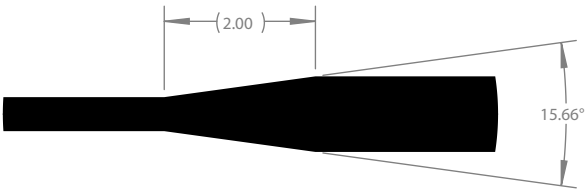
DETAIL B SCALE 10 : 1
