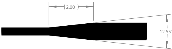
DETAIL B SCALE 10:1
