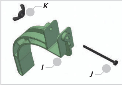
STIRRUP ASSEMBLY
