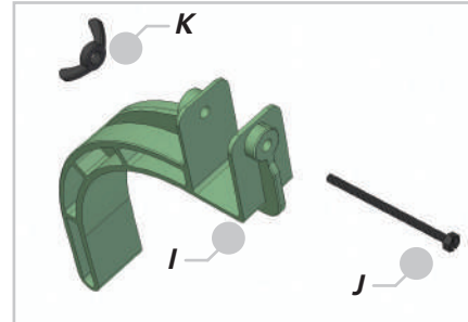
ÉTRIER RAPIDCLIMB
