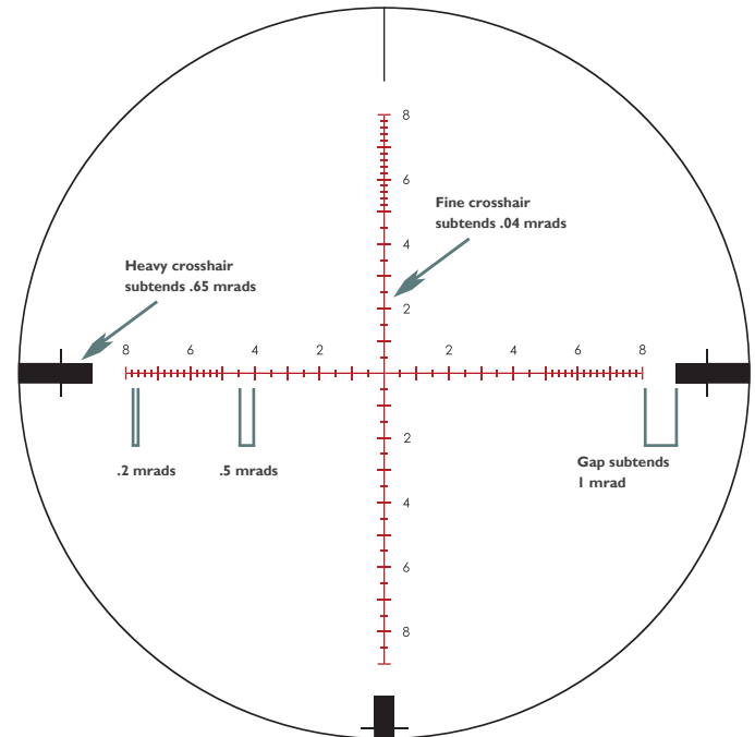
EBR-1 Mrad Reticle Subtensions
